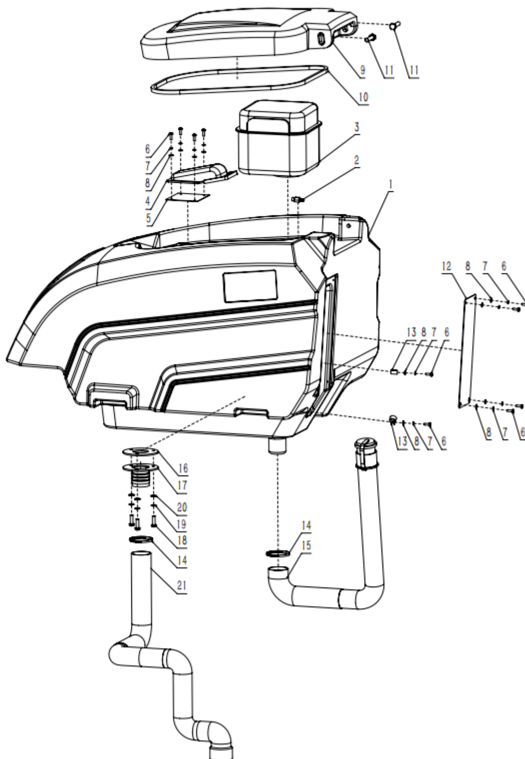
Sewage tank assembly
